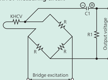
KHCV measuring circuit
